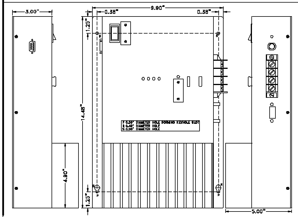
Mechanical Diagram
