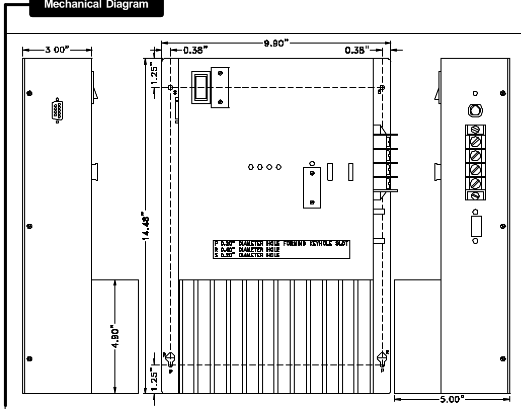
Mechanical Diagram
